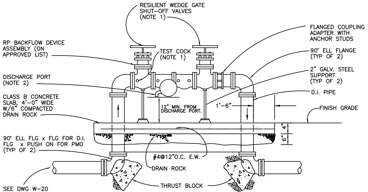
DETAIL A
